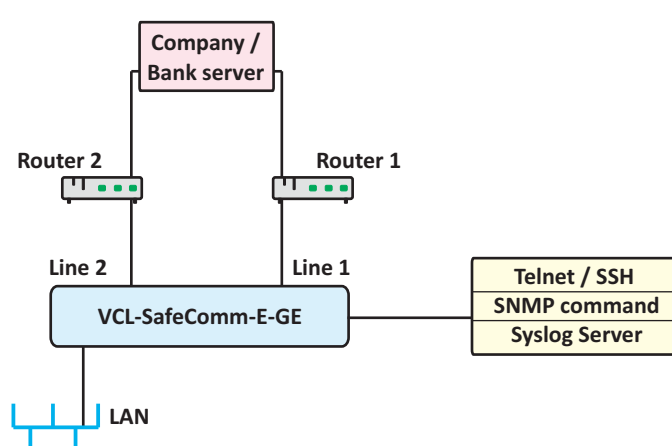
Application Block Diagram #2 (monitoring enterprise server)
