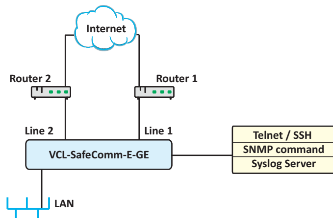
Application Block Diagram #1 (monitoring internet connectivity)
